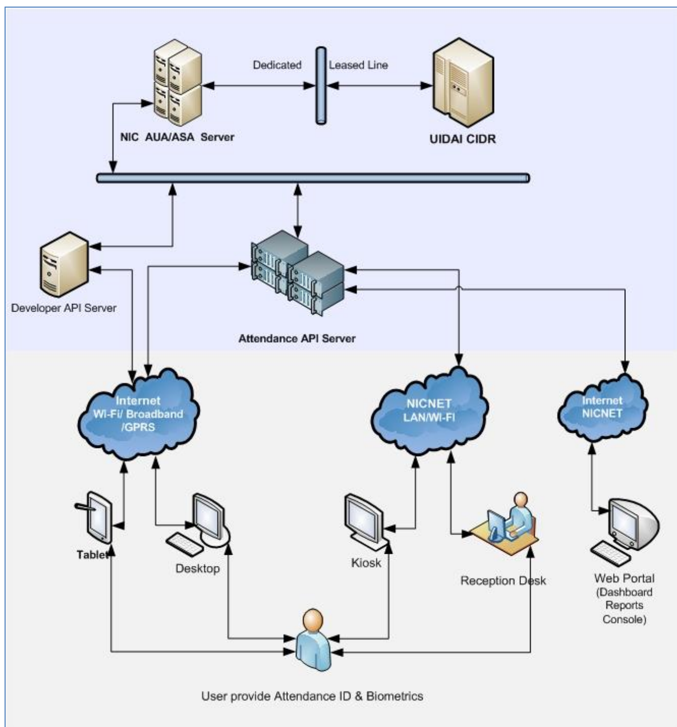
Figure 1: BAS Application Overview
